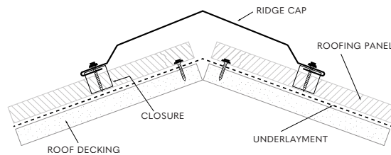
RIDGE CAP
