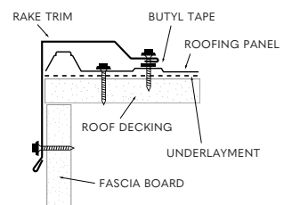
RAKE & GABLE
