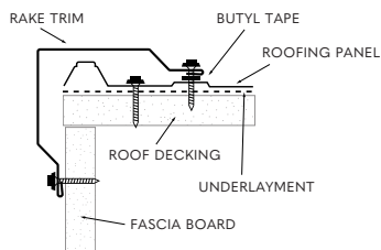
RAKE & CORNER
