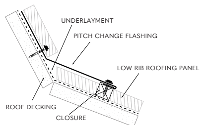
PITCH CHANGE
