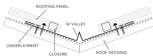
VALLEY
